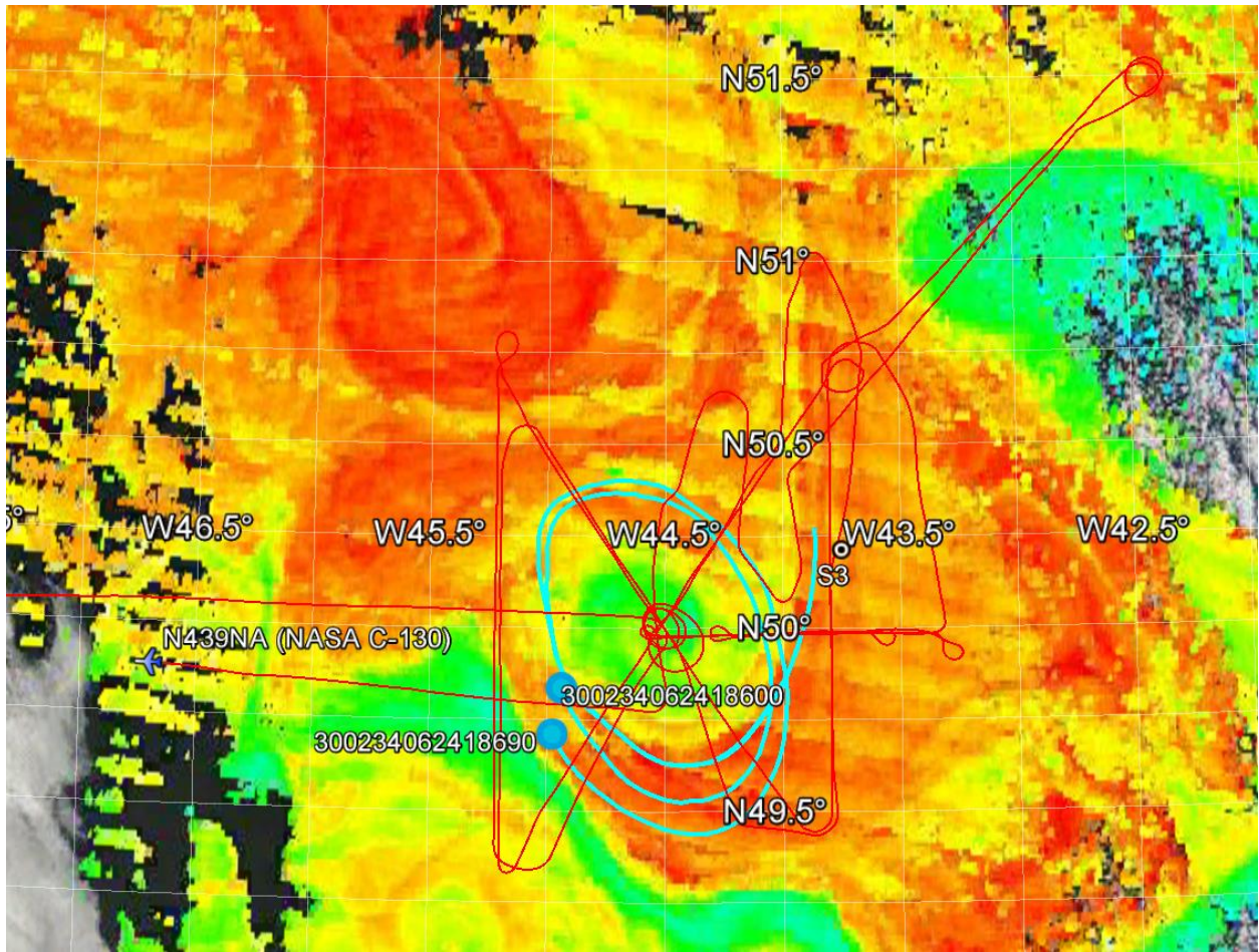
CompleteFlightTrackOverlaidOnTheMay23rdMODISchlMap
